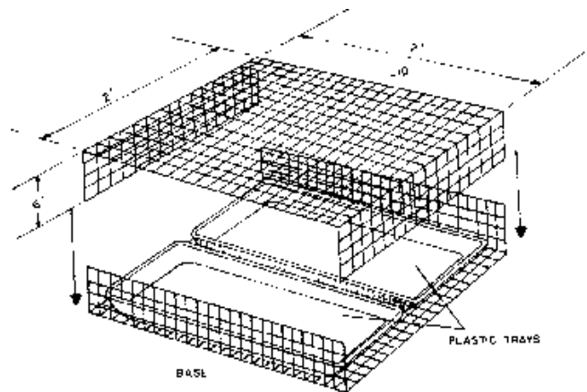
Figure 3. Typical wire cage used for holding giant clams (from Calumpang, 1992).
