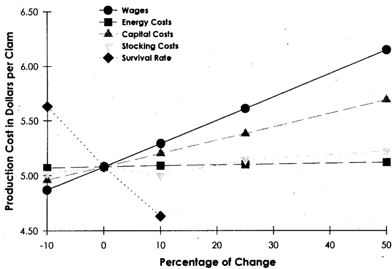
Figure 8. Sensitivity of Production Cost to Changes in Wages, Energy Costs, Capital Costs, Stocking Cost and Survival Rate for the Nursery Phase, Raceway Hatchery System, Republic of the Marshall Islands
